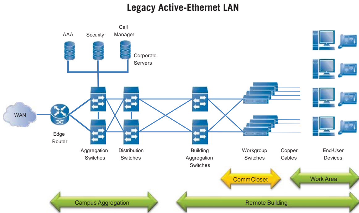
Figure 1. Copper-based LAN systems have a 100-meter limitation that drives a 4-tier network architecture for a typical campus. Workgroup switches are placed on every floor in a building, sometimes in multiple communication closets per floor. Additional switches aggregate the traffic for each building, and in turn, the building aggregation switches connect to campus aggregation and distribution switches which then connect to a router and finally the WAN.
